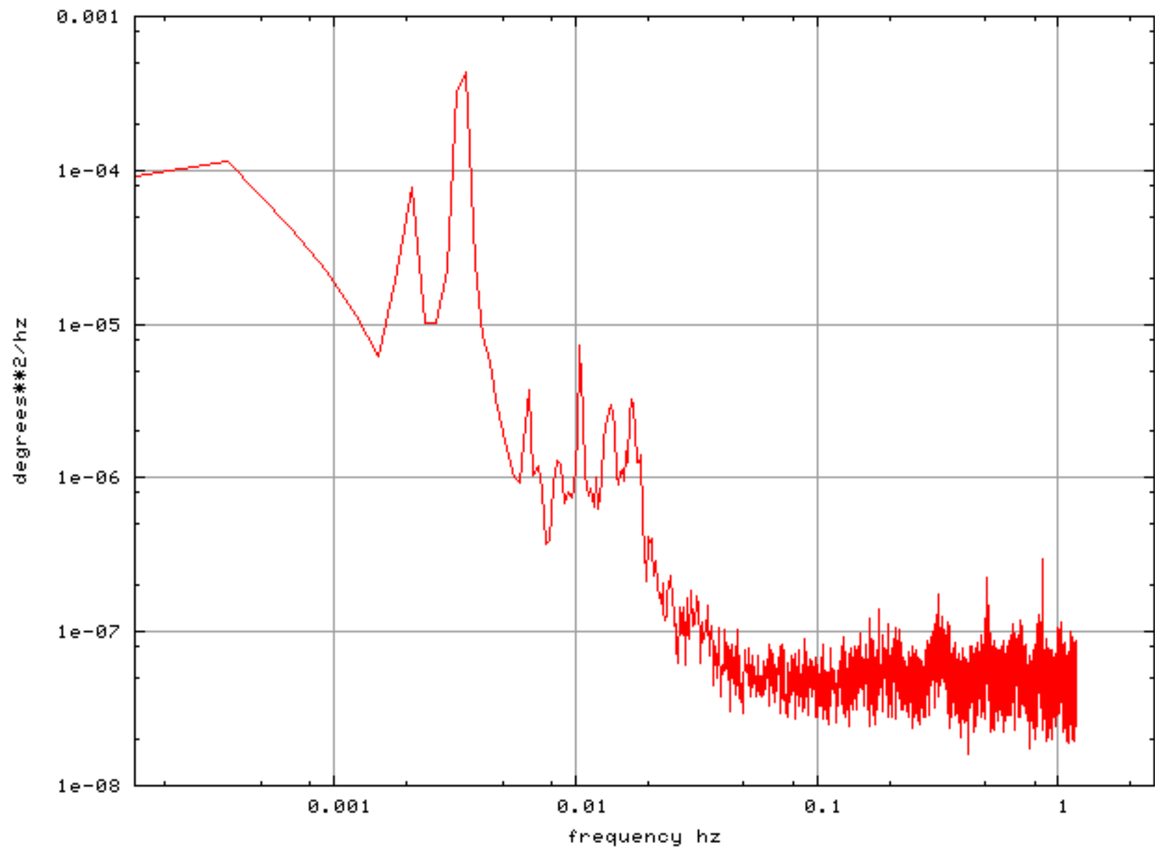
Lucas inclinometer - float: incl2 power spectrum
